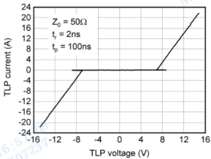
TLP Measurement
