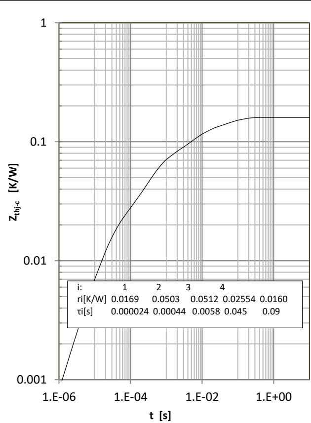
Fig 16. Diode Transient Thermal Impedance
