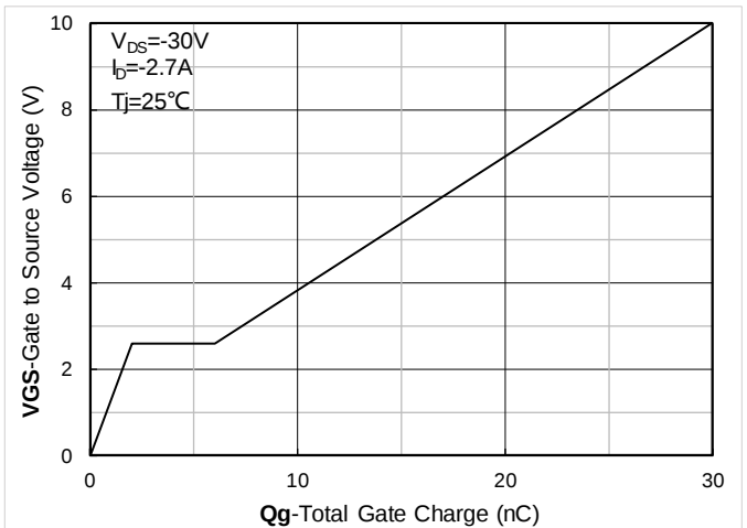
Figure 4. Gate Charge; typical values
