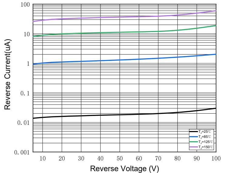
Fig.4: Reverse Characteristics
