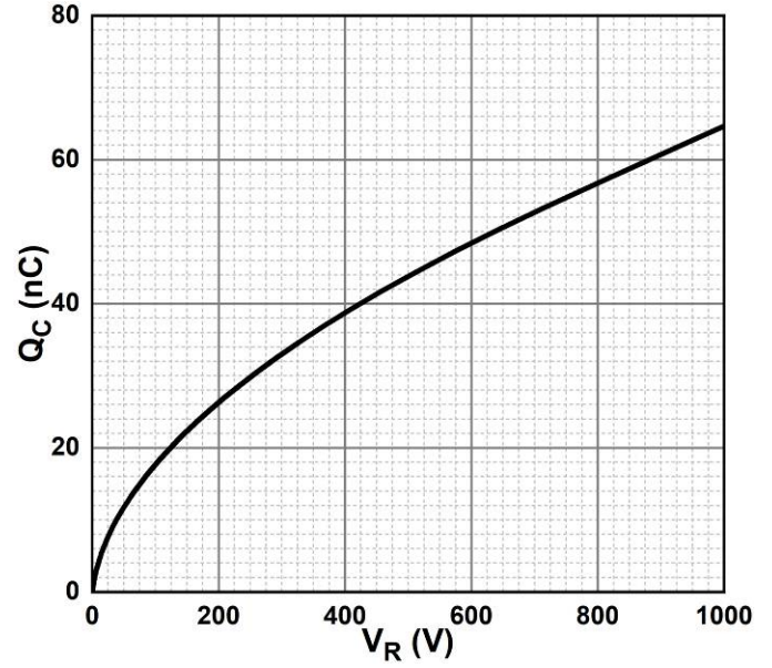
Figure 4. Total Capacitance Charge vs. Reverse
