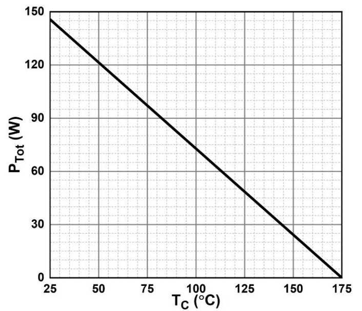
Figure 6. Power Derating
