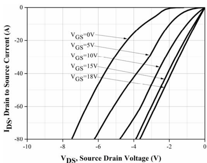
Figure 10. 3 rd quadrant Characteristic at T_j = 25^{\circ}C
