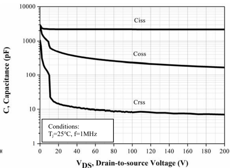
Figure 14. Capacitances vs. Drain Source Voltage (0-200V)
