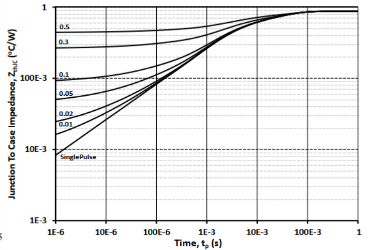
Figure 18 Transient Thermal Impedance (Junction - Case)
