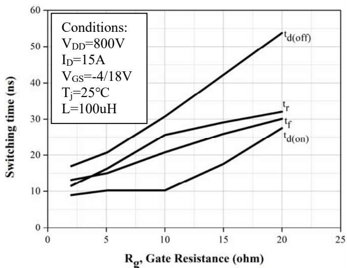
Figure 21. Switching Times vs. R_g
