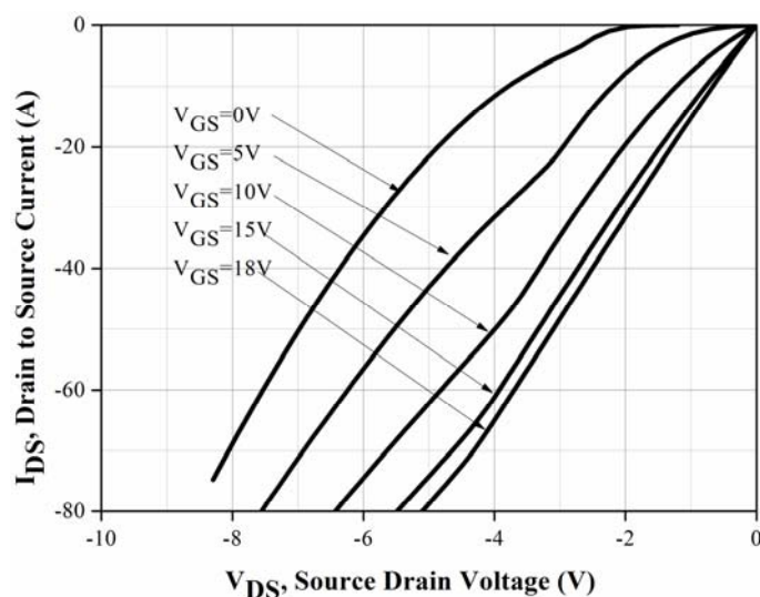
Figure 10. 3 rd quadrant Characteristic at Tj = 25 °C
