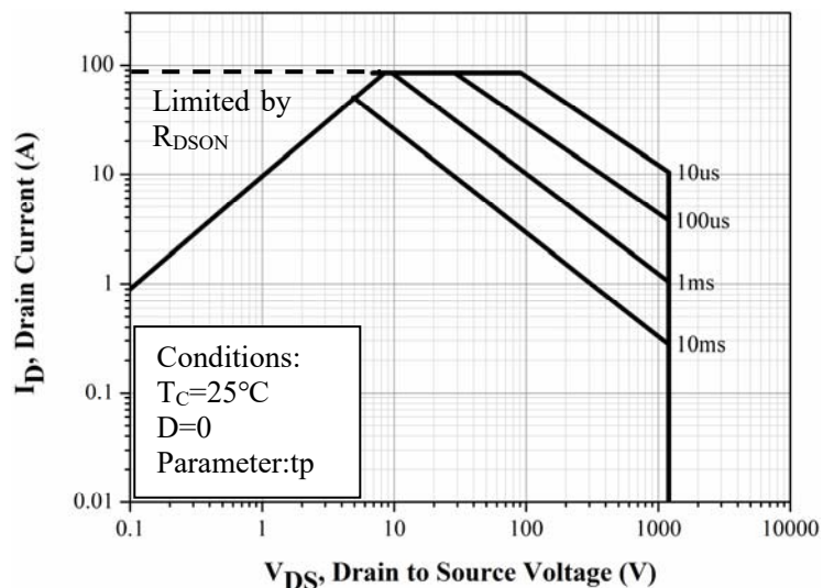
Figure 22. Safe Operating Area
