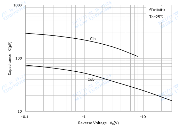
C_{ob}/C_{ib}-V_{CB}/V_{EB}
