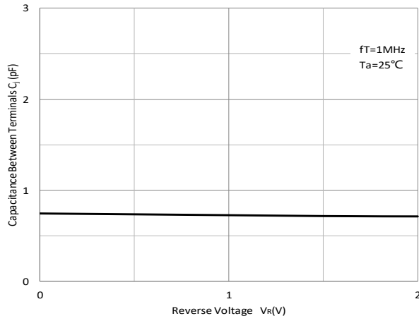
Fig 2: Capacitance Capability
