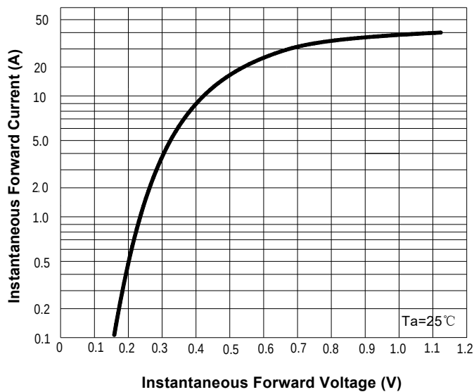
FIG3: Forward Voltage
