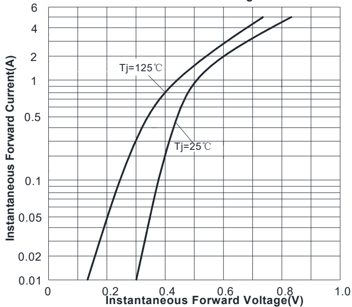
FIG3: Forward Voltage
