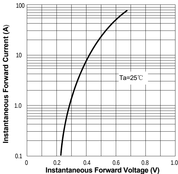
FIG.3: Forward Voltage
