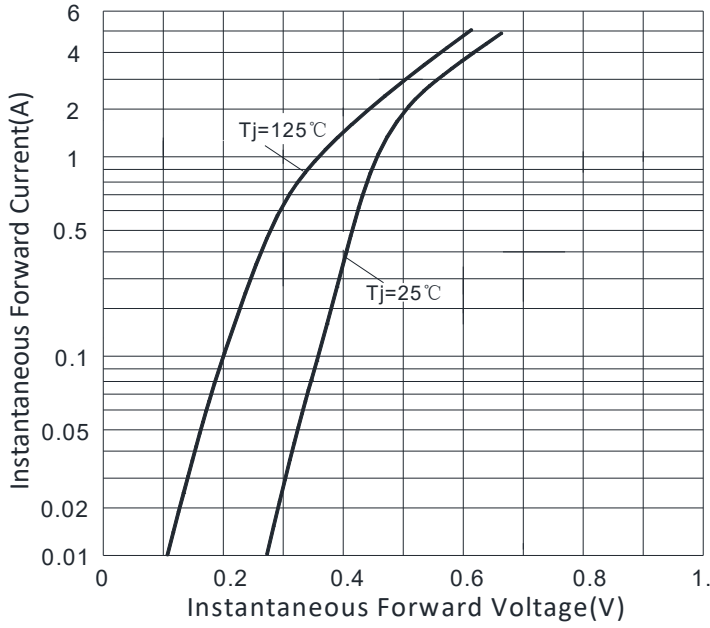
FIG3: Forward Voltage
